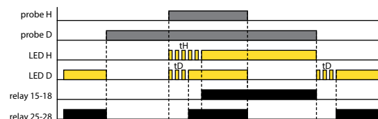
PUMP DOWN, ON DELAY (Function 6)
